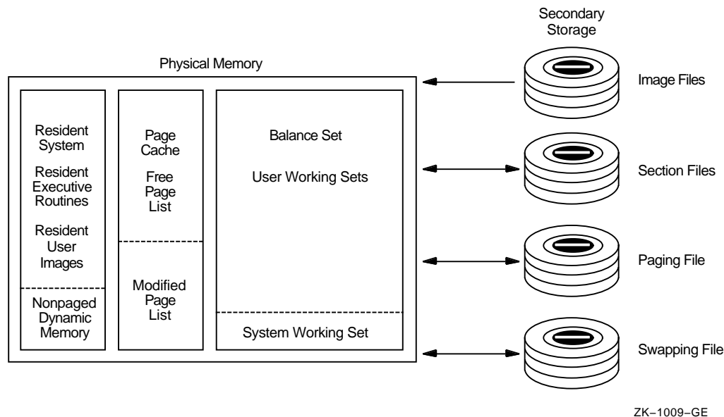
Figure 2-2 OpenVMS Memory Configuration
